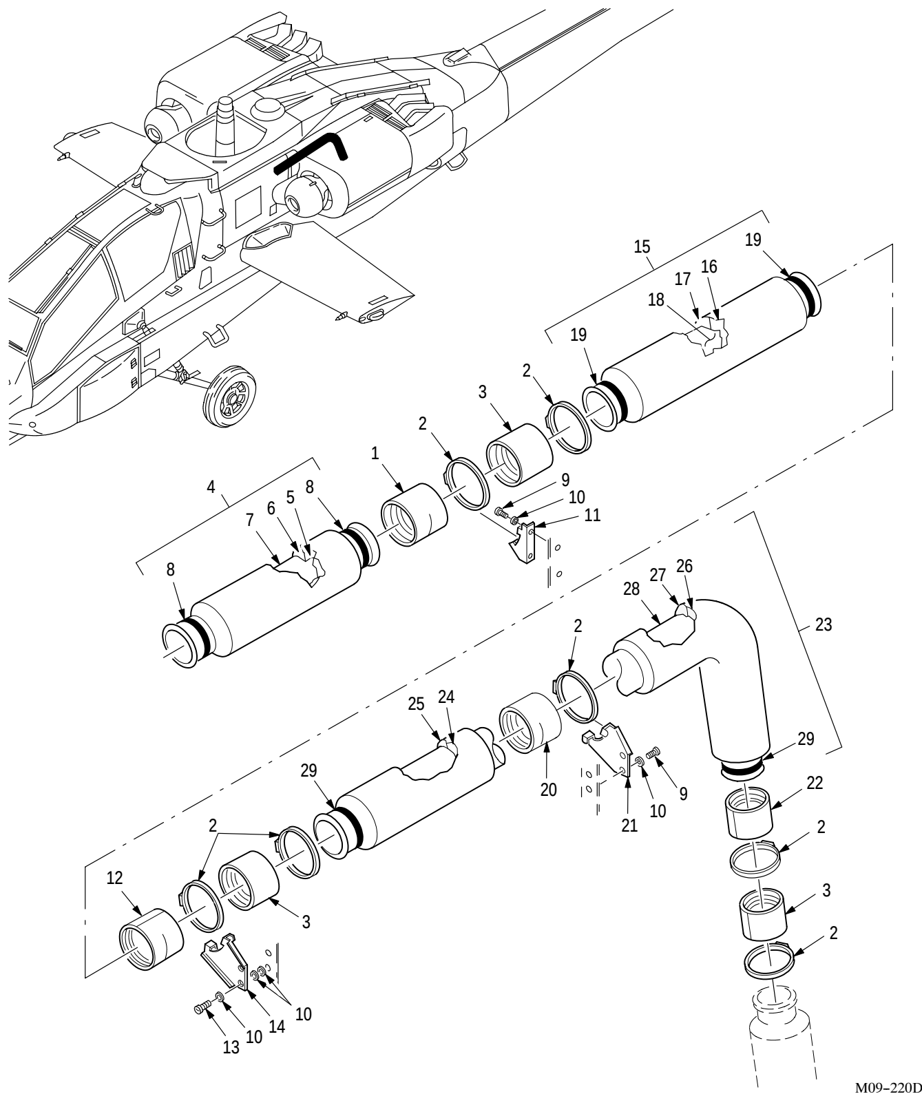
Figure 683. Group 13 Fuselage Environmental Control System (FS 180 to FS 296) 7-311A21100-601
