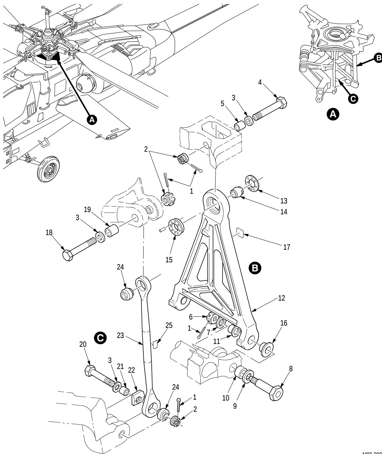
Figure 588. Group 11 Rotor Controls, Upper Main (Torque and Lateral Links) 7-311511100
